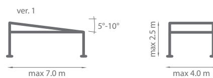
Group installation
