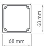
Post cross-section
