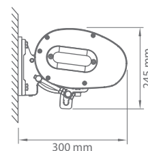
Wall installation
