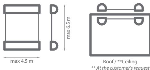
Group installation
