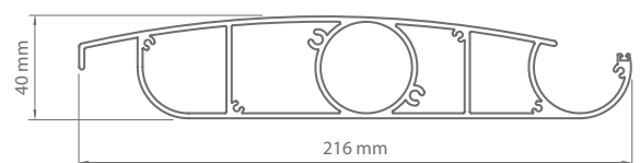
Blade cross-section
