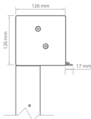
Cassette dimensions
